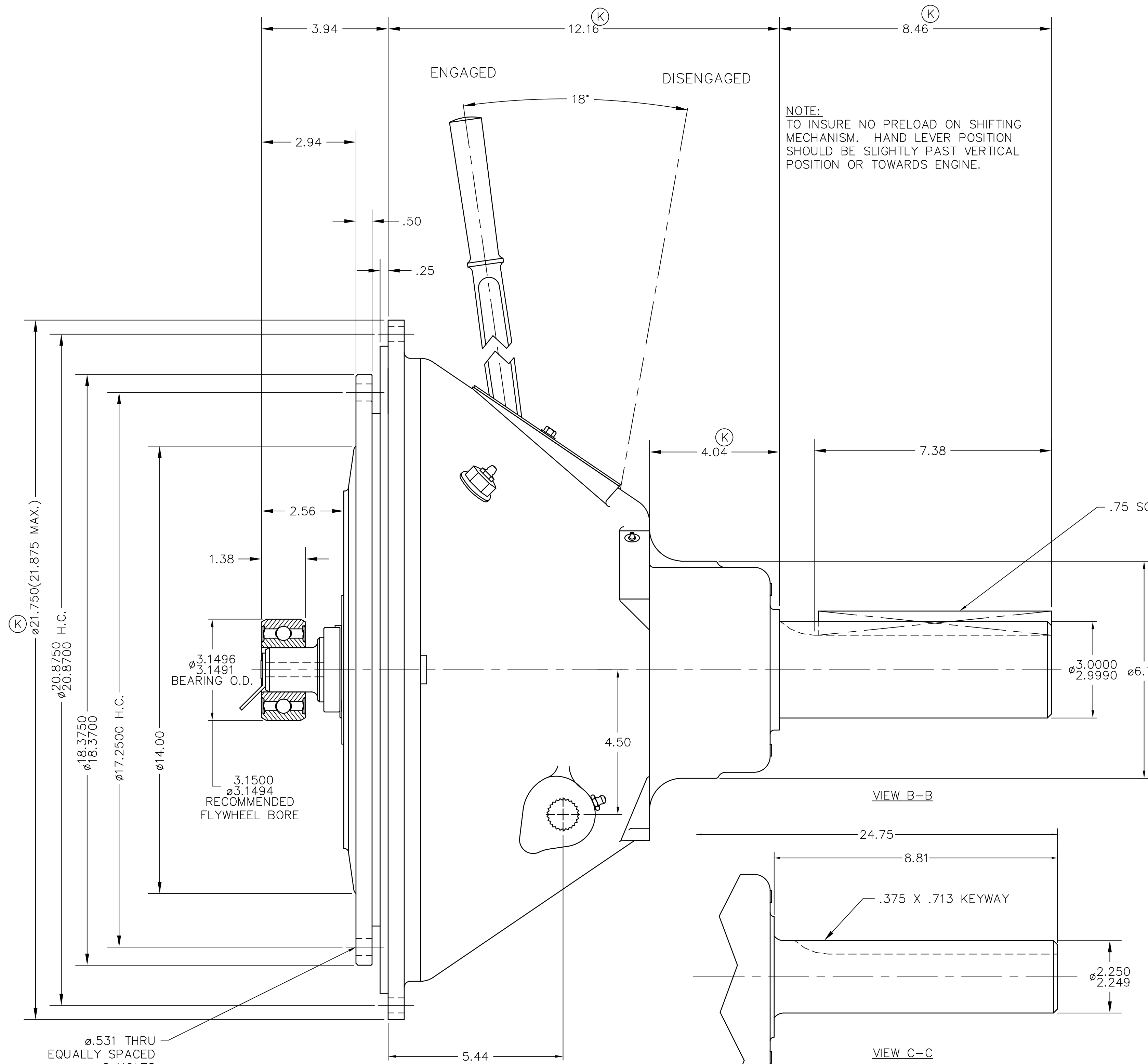
VIEW B-B
