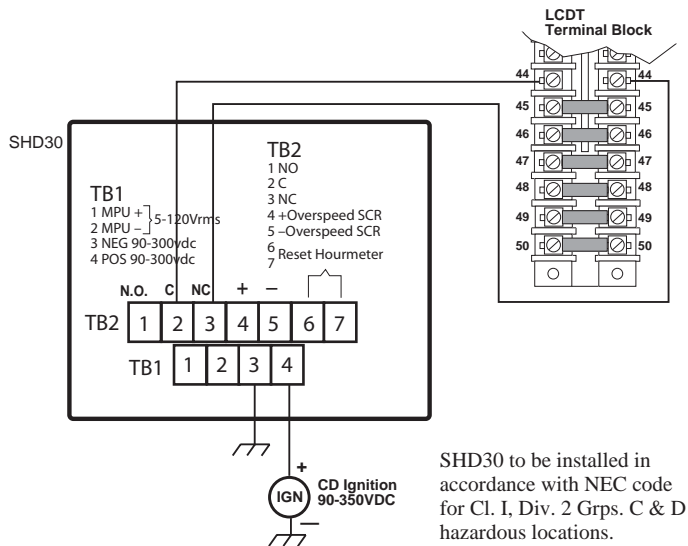
Figure 8: SHD30 models Normally Closed Relay output to LCDT-NC
