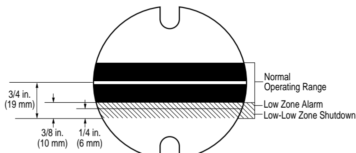
Figure 9: LM304/LM305
